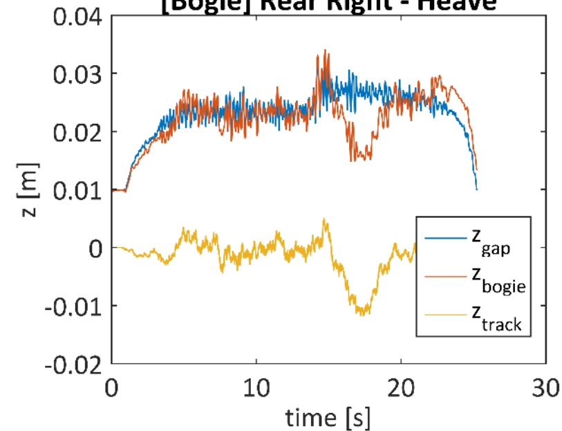
[Bogie] Rear Right - Heave
