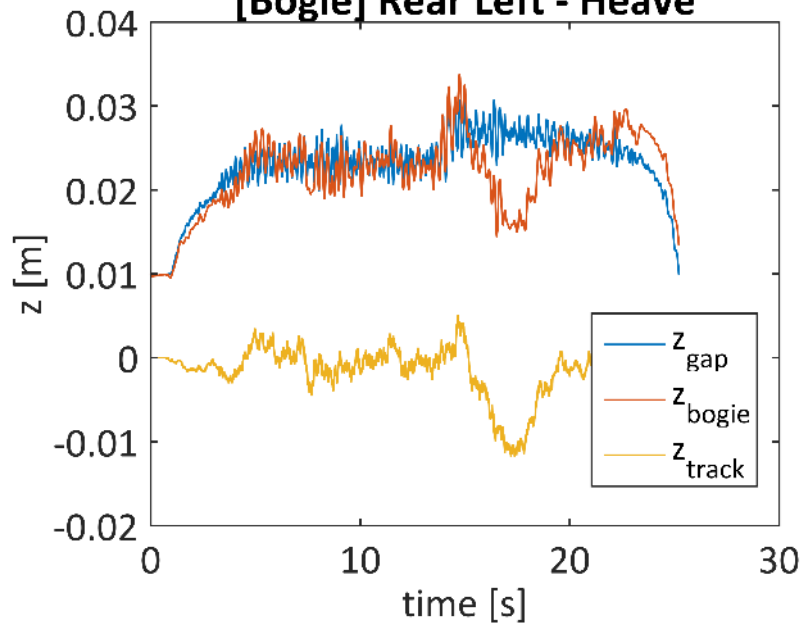
[Bogie] Rear Left - Heave
