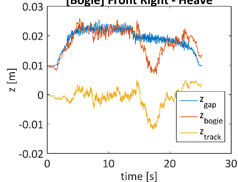
[Bogie] Front Right - Heave
