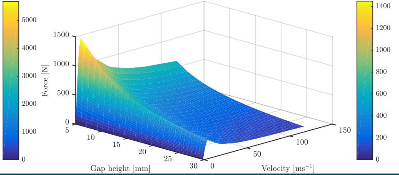
Total drag force
