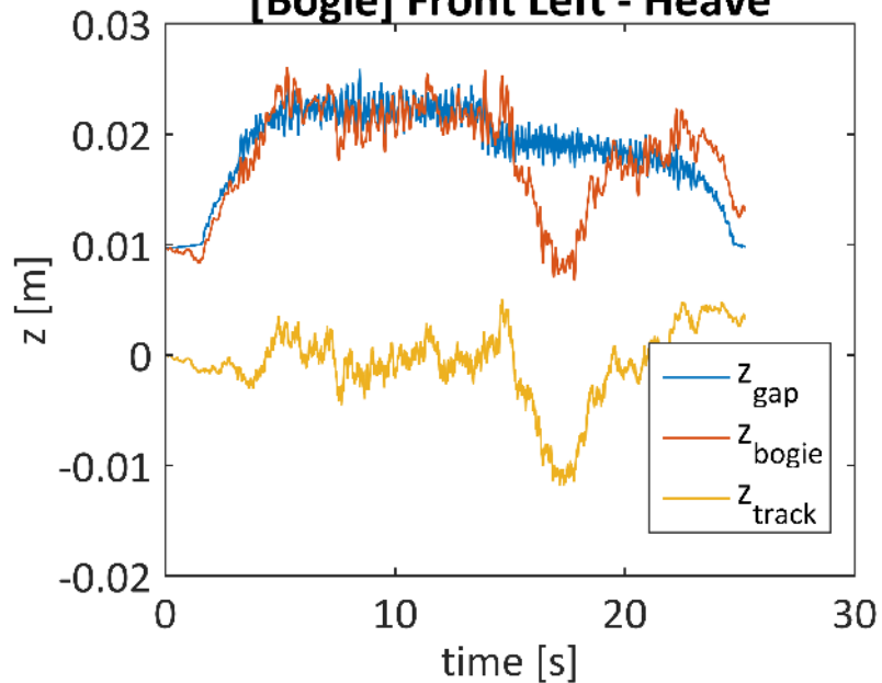
[Bogie] Front Left - Heave
