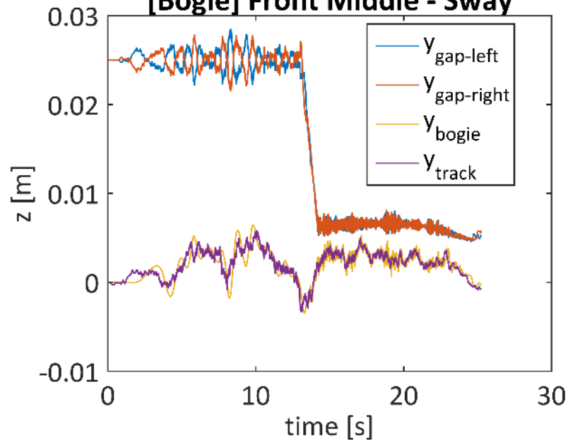
[Bogie] Front Middle - Sway
