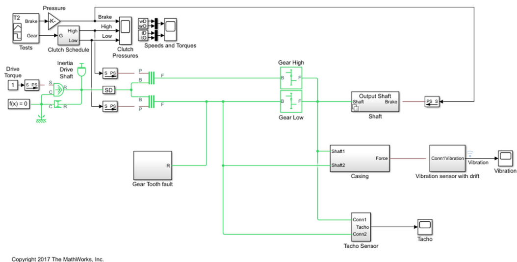
Using Simulink to generate fault data.
